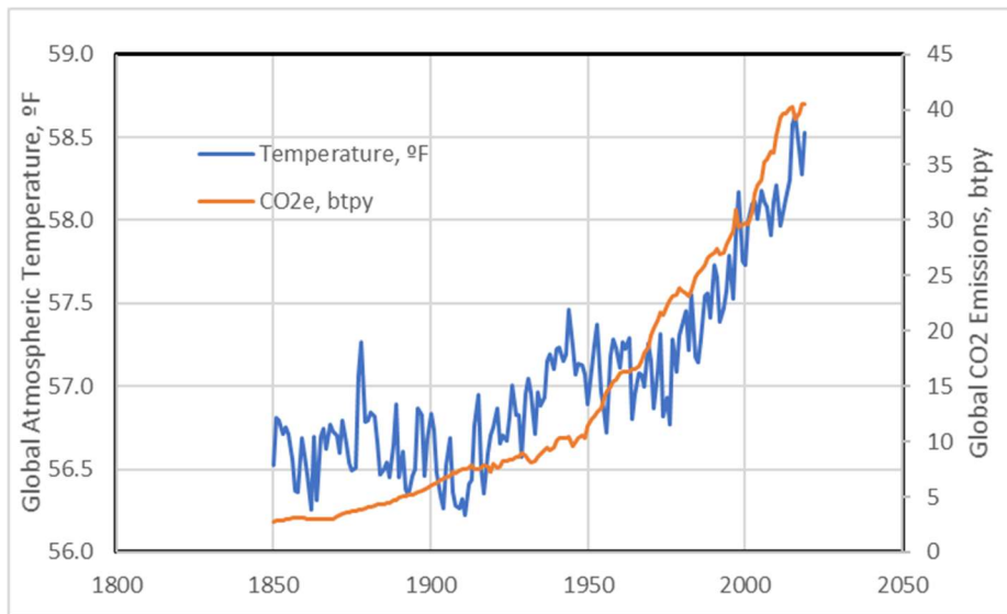
Figure 2 - Atmospheric CO 2 8 and Global Temperature 9 from 1850 to Present.
