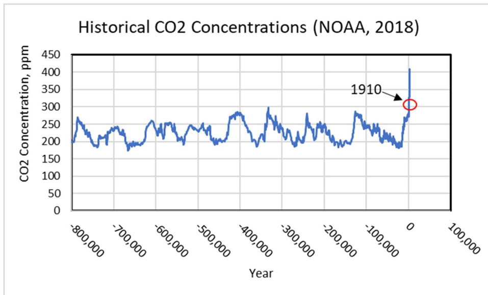
Figure 1 - Atmospheric CO 2 Concentrations from 800,000 B.C. to Present.
